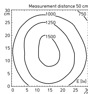
Illuminance with 60° angle of illumination (112 410 003 - 000 698 00)
