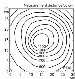
Illuminance with 25° lens
